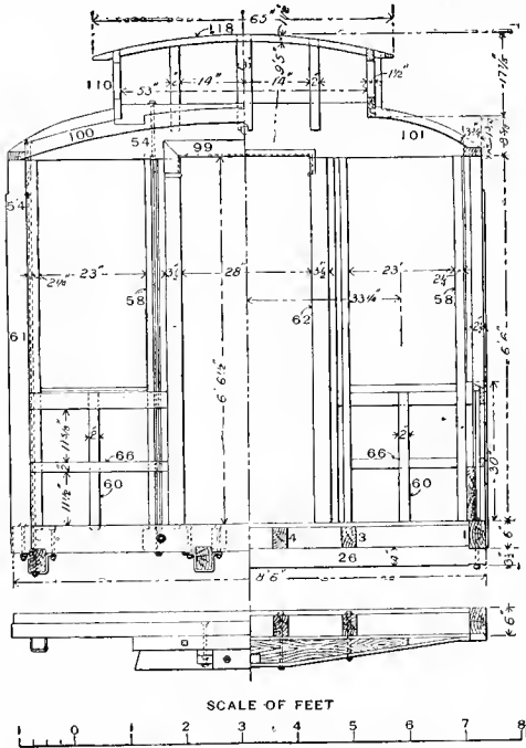
Fig. 465. End Elevation of Framing.
